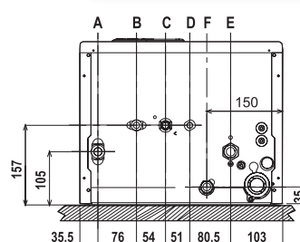
Bottom view TECH C
