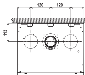
Top view TECH (all models)
