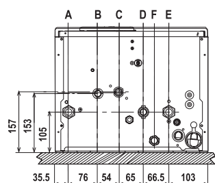
Bottom view TECH A
