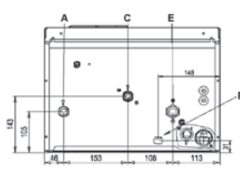
Bottom view TECH H
